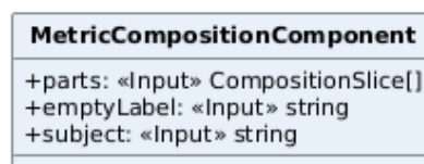
Figura 117: Classe — MetricCompositionComponent
